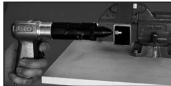
1/4 turn the fastener onto the ARO tool mandrel and place the fastener into the hole.
